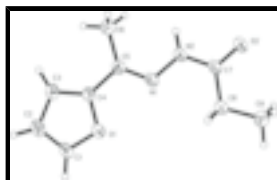
Fig. 1. Structure of the title compound at 30% probability displacement ellipsoids showing the atom-numbering scheme.
